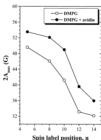
Fig. 5. Positional dependence of the outer hyperfine splitting, 2A_{\max} , for phosphatidylcholine spin labels, n -PCSL, in DMPG membranes (○) and in DMPG/avidin (1:5, w/w) complexes (●), at 30°C, corresponding to the fluid-phase region of DMPG alone.
